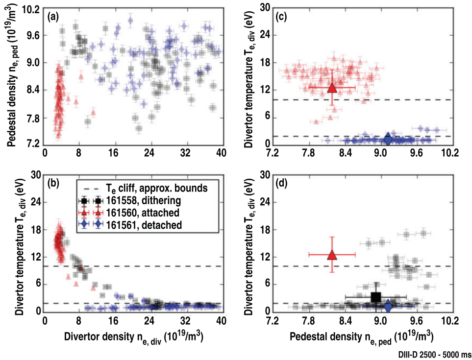
Figure 9. Upstream pedestal density (a) and divertor T_e (b) versus divertor n_e , showing that (a) divertor density can vary widely for the same pedestal density. (c) Divertor T_e versus upstream n_e for the steady attached (red triangle) and detached (blue diamond) cases with time averaged values marked with larger, darker symbols (compare with top/bottom of cliff in figure 2). (d) Divertor T_e versus upstream n_e for the dithering case with time averaged value marked with a larger darker square and averages from (c) overlaid for reference; note that the black squares do not trace out the path suggested by the red triangle, the blue diamond, and figure 2. Dashed lines are drawn at 2 and 10 eV for reference.
