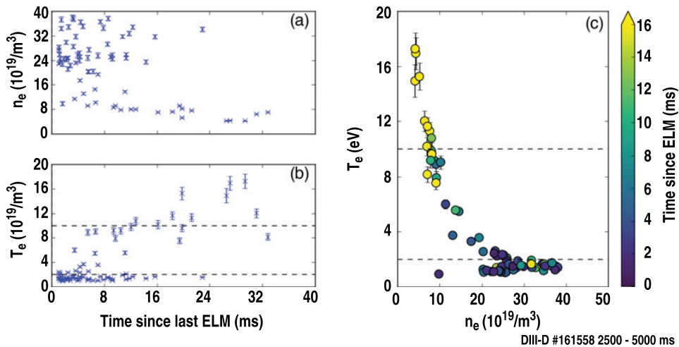
Figure 12. Changes in divertor T_e and n_e versus time since the end of the last ELM. T_e and n_e are measured by DTS at the control chord shown in figure 3. (a) and (b): n_e and T_e versus time since last ELM. (c): T_e versus n_e with symbols colored by time since last ELM. Dashed horizontal lines mark the approximate edges of the T_e cliff at 2 and 10 eV. Attached samples typically occur longer after ELMs. The scatter the length of the detached phase after ELMs probably results from variability in the ELMs themselves and adjustments to gas flow made by the control system. In particular, the single cold, dense point occurring 24 ms after the last ELM (yellow mark at bottom right of (c)) was measured at 2936 ms, just after a period of aggressive puffing when T_e stayed cool for about half a second without dithering (see figures 5(c) and (d)).
