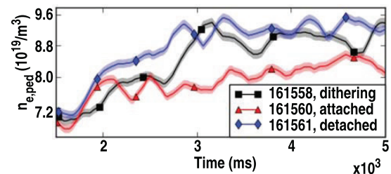
Figure 6. Comparison of upstream pedestal density for different detachment conditions with control starting at 1.5 s. Pedestal density is calculated from automatic tanh fits [16] to Thomson scattering [10] and is filtered to remove measurements taken during ELMs. The control setting for the detached case (blue diamonds, T_e request = 2.0 eV) leads to more aggressive initial gas puffing than the dithering case (black squares, T_e request = 5.0 eV), but both of these cases have reached about the same density by 3 s. The attached case (red triangles, T_e request = 12.0 eV) stays at lower density.
