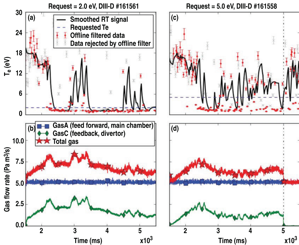
Figure 5. Measured versus requested T_e at the divertor target versus time ((a) and (c)) and gas flow rates ((b) and (d)) for request = 2 eV (detached) ((a) and (b)) and request = 5 eV (dithering) ((c) and (d)). (a) and (c) Black: time history of real time filtered and RC low-pass smoothed Thomson T_e measurements. Red points: post-shot filtered and cleaned up T_e measurements; these agree well but not perfectly with the real time filtering as the post-shot filter is more complex and can be inspected and fine-tuned more easily. Blue dashed line: requested T_e value. (b) and (d) Constant gas puff into the main chamber to maintain baseline density (blue squares), feedback controlled gas puff into divertor (green diamonds), and total gas puff (red stars).
