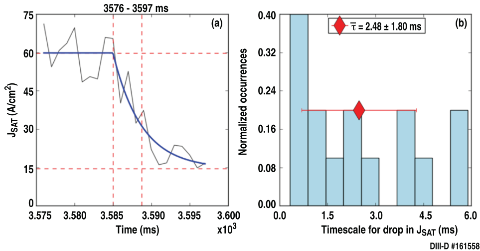
Figure 11. (a) Example of exponential fit to J_{\text{sat}} versus time during re-attachment; measured J_{\text{sat}} is shown in black while the fit is shown in blue. (b) Histogram of results from timescale fits to several reattachment events. The selected events were those which occurred during quiescent periods between large ELMs. One outlier ( \tau = 12 ms) out of 16 measurements was discarded, giving an average timescale of 2.48 ms with standard deviation of 1.8 ms (with the outlier, the average is 3.26 \pm 2.89 ms). The average value and standard deviation are marked on the plot by the red diamond with error bars.
