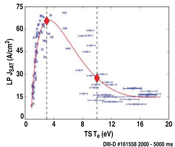
Figure 10. Saturation current density ( J_{\text{sat}} ) from Langmuir probes versus electron temperature ( T_e ) from divertor Thomson scattering at the control chord. The approximate edges of the T_e cliff are marked by red diamonds; note the limited data between the diamonds (compare with figure 7).
