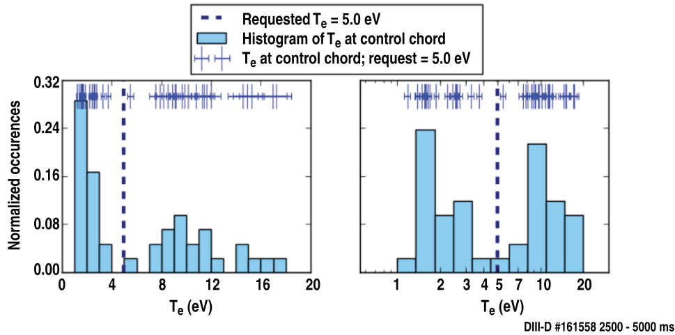
Figure 7. Histogram (bars) of T_e measurements (symbols) at the divertor target (see figure 3) during control with a request in the middle of the cliff (dashed line), shown with linear (left) and logarithmic (right) X -axis scaling. The data separate into two groups around 1–3 eV and 8–20 eV with a sparse region near the requested value. The logarithmic bin spacing in the right panel is useful for visualization because of the difference in width of the two groups; presumably the group widths differ because higher temperature plasmas experience greater fluctuations in T_e , or DTS uncertainty and thus scatter in measurements is higher (this can be seen from the plot where error bars are roughly constant width in the right panel but get wider at higher T_e in the left panel), or both. DTS uncertainty is higher at higher temperature only because density is lower (see figure 12 for correlation between n_e and T_e ) and thus signal to noise is lower.
