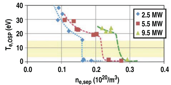
Figure 2. DIII-D divertor T_e from Thomson scattering parameterized against upstream separatrix density for three steps in a power scan, showing the T_e cliff marked by the yellow shaded region. Curves are drawn through the data to guide the eye. Reprinted from [5], Copyright 2015, with permission from Elsevier.
