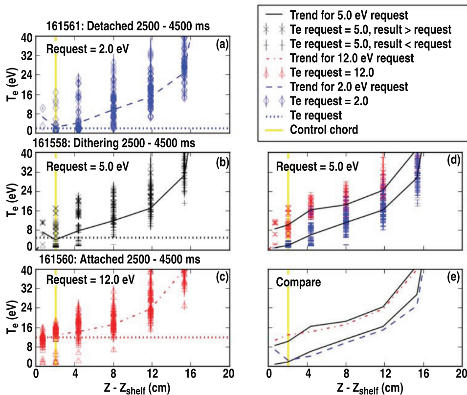
Figure 8. Profiles of electron temperature versus height above the shelf for three requested T_e values representing detachment, attachment, and dithering across the T_e cliff. See figure 3 for the relationship between the Thomson measurement locations and the magnetic flux surfaces. The lowermost Thomson chord (left of the plot range, Z - Z_{\text{shelf}} = 0.7 cm) was not used for control due to the impact of stray light from the edges of the laser hole (see the sparsity of measurements for the left-most chord in (a)); instead the next lowest chord at Z - Z_{\text{shelf}} = 2 cm was used (marked by the dashed green vertical line). Three shots are shown: (a) request = 2 eV, plasma stayed detached most of the time, (b) request = 5 eV, dithering detachment/re-attachment, and (c) request = 12 eV, plasma stayed attached most of the time. Trends are obtained by weighted average of all the data from each chord. The trendlines in all three cases ((a)–(c)) are consistent with the requests to the controller (they go through the intersection of the dotted green lines). As T_e at the control chord in (b) is jumping across the T_e cliff, we separate the data in (b) into two groups according to T_e > \text{request} or T_e < \text{request} and plot these with separate trendlines in (d). (e) Compares the trendlines from (a) and (c) to those in (d), showing that the dithering shot is jumping between the T_e profiles observed in the two steady shots at the hot and cold edges of the cliff, and that the entire profile jumps rigidly between states.
