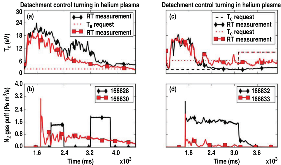
Figure 13. Initial deployment of the detachment controller in a new scenario ((a) and (b)) and performance of the feedback detachment controller with nitrogen puffing into helium plasma ((c) and (d)). (a) and (c) Real time temperature measurements (solid) and requested values (dashes); the request in (c) is increased in the latter half of the flattop. (b) and (d) N_2 gas flow rates; the gas flow in 166828 (black in (a)) was the tuning data acquisition shot and was the only one not under feedback control. The initial spike in gas flow is added to ensure that the valve does not stick closed when starting with small flow commands.
