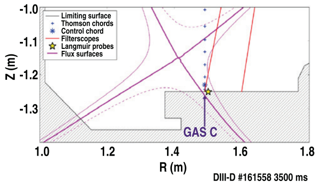
Figure 3. Positions of diagnostics and actuators for the detachment control system in the lower divertor region of DIII-D. Of the filterscope chords shown, the outermost was used for detecting ELMs during detachment as the normally prominent ELM-induced flash of light at the strike point is not as clear in detached plasmas and can actually become inverted in deep detachment. However, both chords were connected to the PCS and available in real time. The location of the Langmuir probe used later (section 3.1.1) is shown as well. Of the available DTS chords, the favored one for use in the control system is marked with an asterisk and reported T_e will be from this chord unless otherwise specified.
