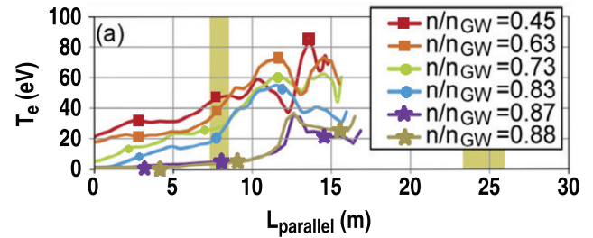
Figure 1. Profiles of T_e versus L_{\text{parallel}} , the distance along the field from the target plate, averaged over the flux surface range of \psi_N = 1.000\text{--}1.004 . The attached profiles are marked with red and orange squares, partial detached profiles with green and blue circles, and fully detached profiles with purple and brown stars. The vertical shaded regions mark the X-point and the outboard midplane. Measurements are from DIII-D's divertor Thomson system [8]. The apparent peaking behavior around L_{\text{parallel}} = 13 m may be related to poloidal variation in electron pressure reported by Shaffer et al [9] (see figure 9 of [9]). Although Shaffer's model detected variation in density, perhaps similar effects influence T_e . There may be other explanations, such as scatter in the measurements. Reprinted from [5], Copyright 2015, with permission from Elsevier.
